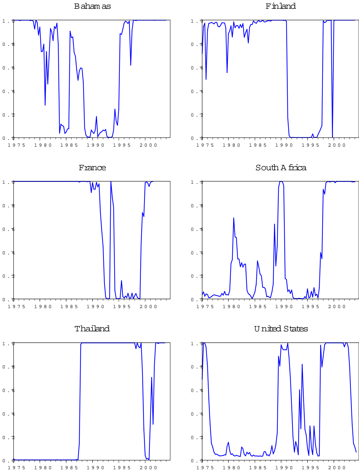
Figure 2: Regime 1 filtered probabilities
